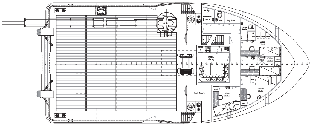
Main Deck
